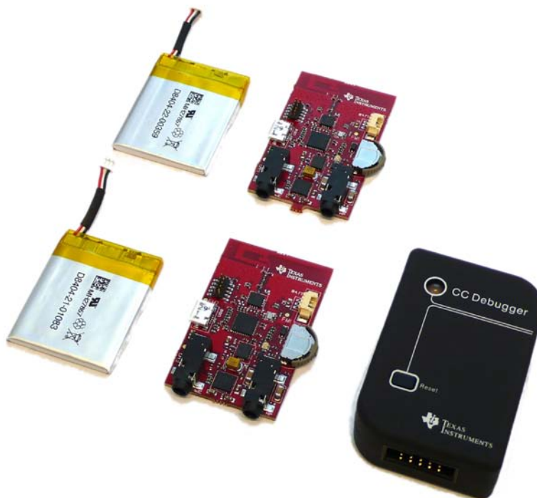
Figure 1. The main components included in the PurePath Wireless Headset Kit.
