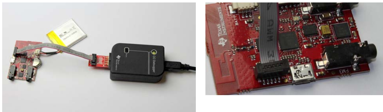
Figure 3. CC debugger connected to the CC85xx Headset board
